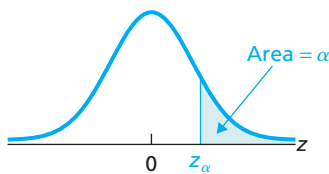
FIGURE 6.14 The z_\alpha notation
