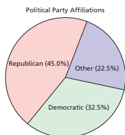
FIGURE 2.2 Pie chart of the political party affiliation data in Table 2.1
