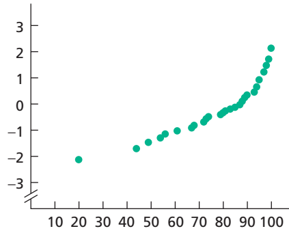
FIGURE 9.22 Normal probability plot and stem-and-leaf diagram for Problem 30
