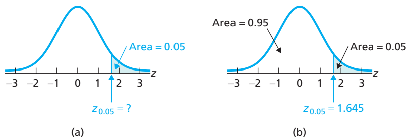
FIGURE 6.16 Finding z_{0.05}
