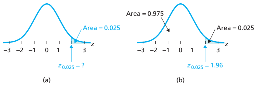
FIGURE 6.15 Finding z_{0.025}
