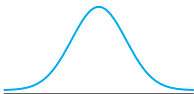
FIGURE 6.1 A normal curve
