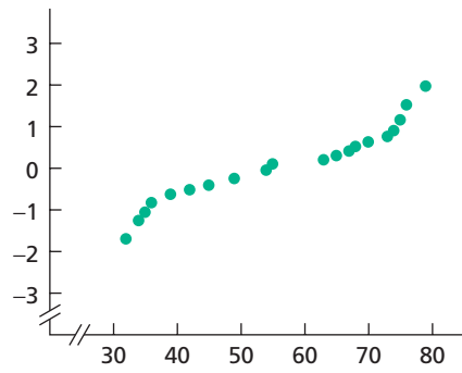
FIGURE 9.26 Normal probability plot and stem-and-leaf diagram for Problem 34
