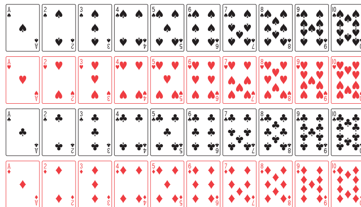
FIGURE 5.10 Event (\text{not } D)
