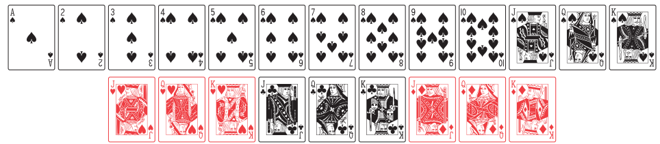
FIGURE 5.20 Event E
