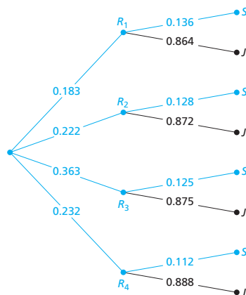
FIGURE P.7 Tree diagram for calculating P(S) , using the rule of total probability
