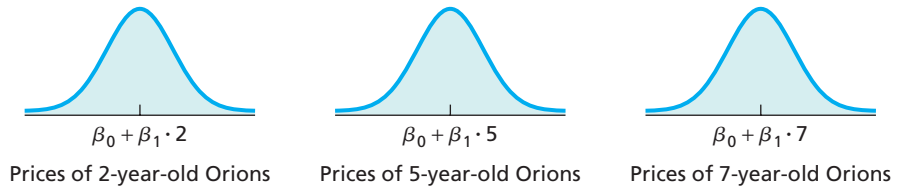
FIGURE 14.3 Graphical portrayal of Assumptions 1–3 for regression inferences pertaining to age and price of Orions
