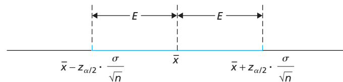
FIGURE 8.7 Margin of error, E = z_{\alpha/2} \cdot \frac{\sigma}{\sqrt{n}}
