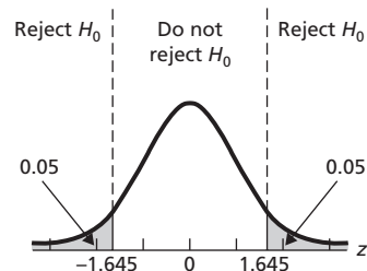
f. Two-tailed test
