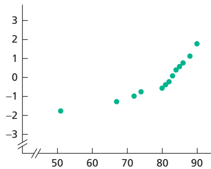
FIGURE 9.29 Normal probability plot and stem-and-leaf diagram for Problem 37
