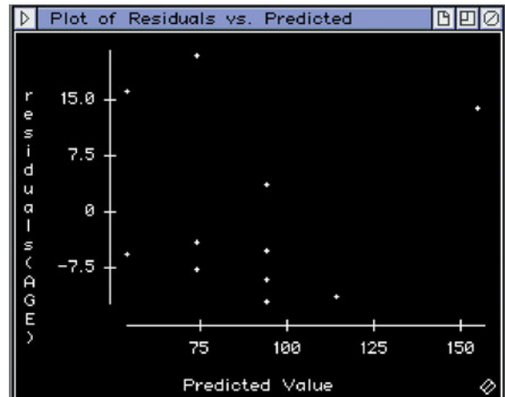
OUTPUT 14.1 Residual plots and normal probability plots of the residuals for the age and price data of 11 Orions
