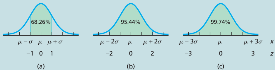
FIGURE 6.20 The 68.26-95.44-99.74 rule
